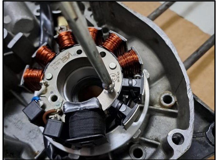
3- Fasten the coil plate and the coil in the shown position.
